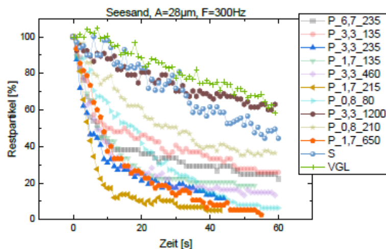
Figure 3: Measurement of residual particles left on different artificial samples over time. The excitation used in this experiment had a frequency of 300 Hz and amplitude of 28μm. Some combinations of step height and periodicity are superior to others.
