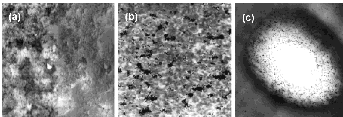
Figure 6. (a) Scanning electron micrograph (SEM) showing the interior of a palladium diacetate containing polyurea microcapsule (magnification 3 \times 2500 ). (b) TEM of a sliced palladium diacetate microcapsule after chemical reaction (magnification 3 \times 14,000 ). (c) TEM of a sliced microcapsule showing the distribution of palladium nanoparticles (dark spots) along a channel formed within the polyurea matrix (magnification 3 \times 46,000 ).
