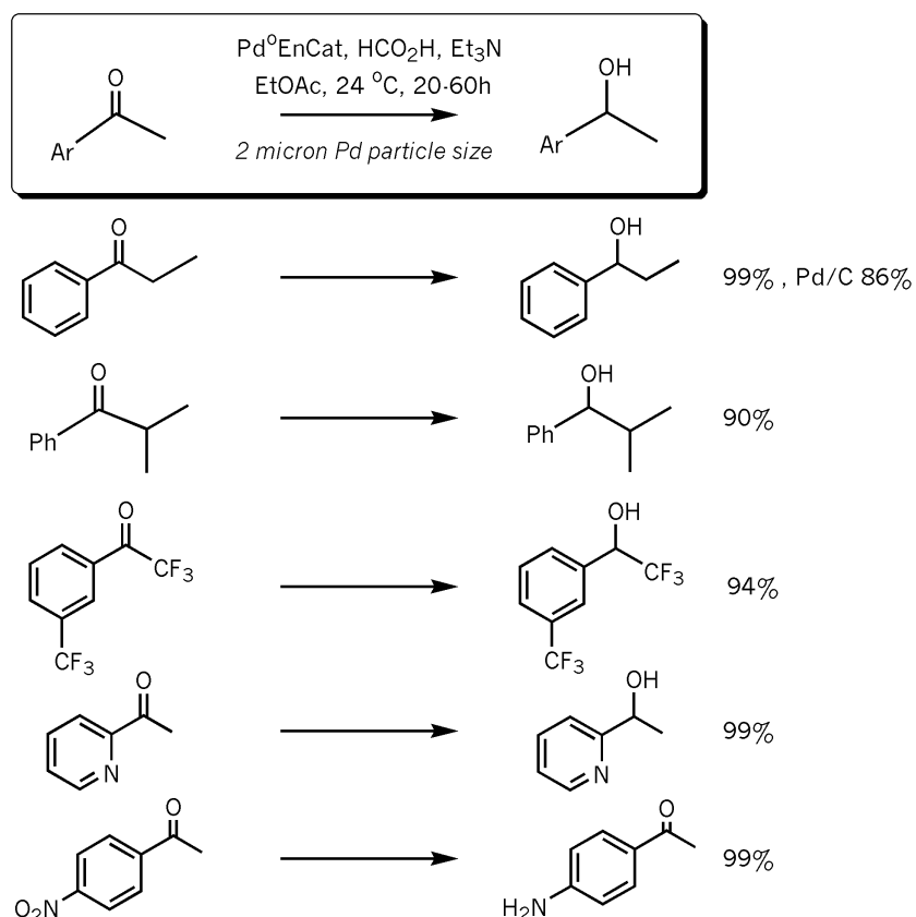
Figure 10. Micro-encapsulated Pd(0) for hydrogenation transfer reduction of aryl ketones.
