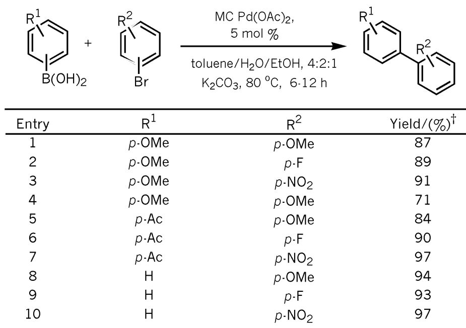
Figure 7. Synthesis of biaryls using palladium diacetate encapsulated in polyurea.
