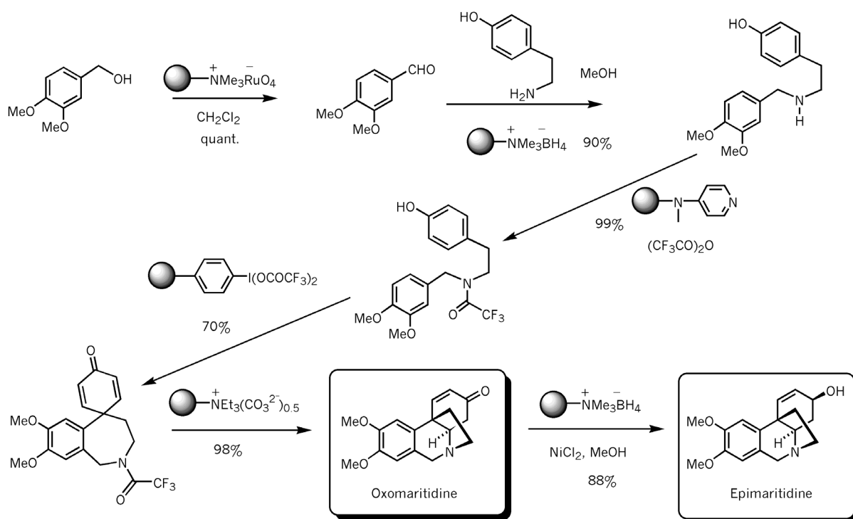
Figure 17. Synthesis of (±)-oxomaritidine and (±)-epimaritidine.
