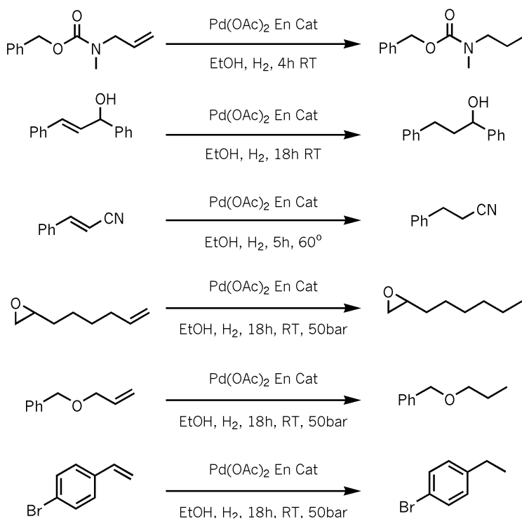
Figure 9. Palladium diacetate En Cats in hydrogenation reactions.
