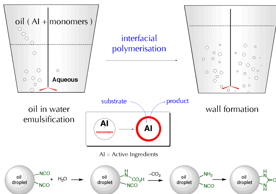
Figure 5. Microcapsule manufacture by interfacial polymerisation.
