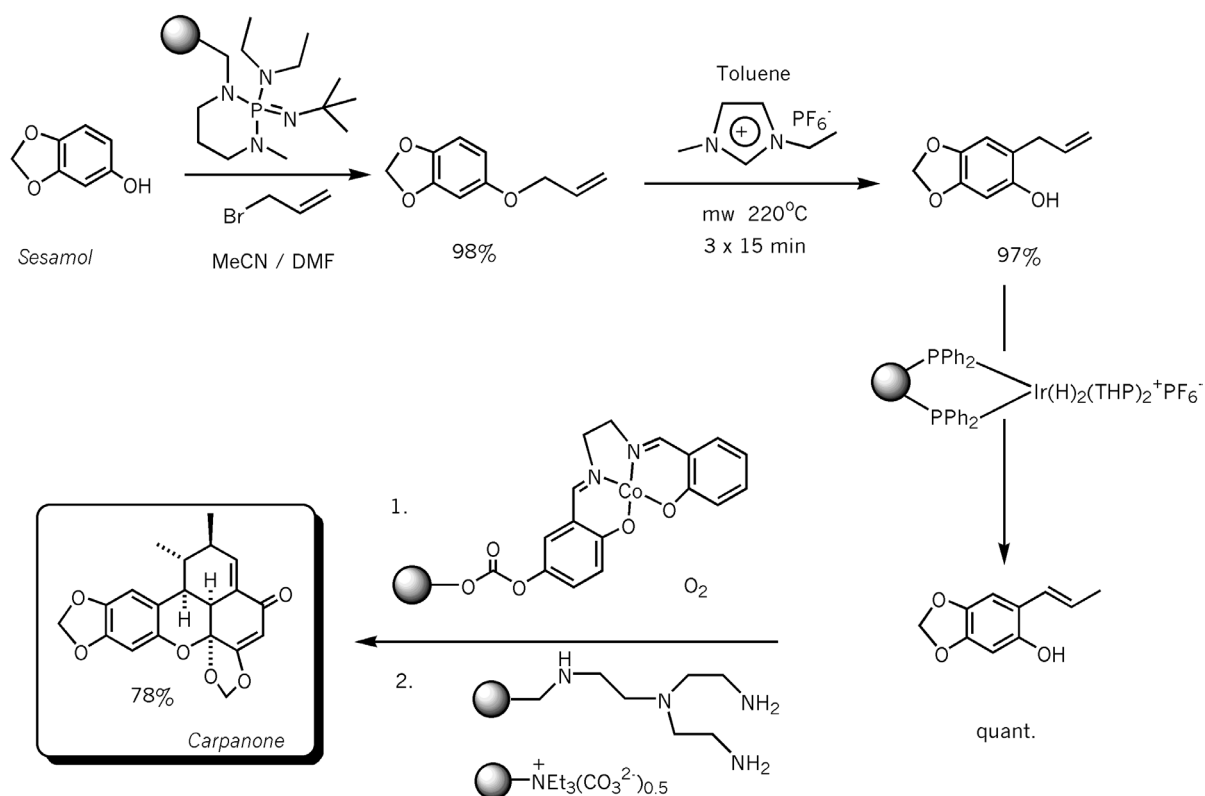
Figure 16. Synthesis of carpanone.
