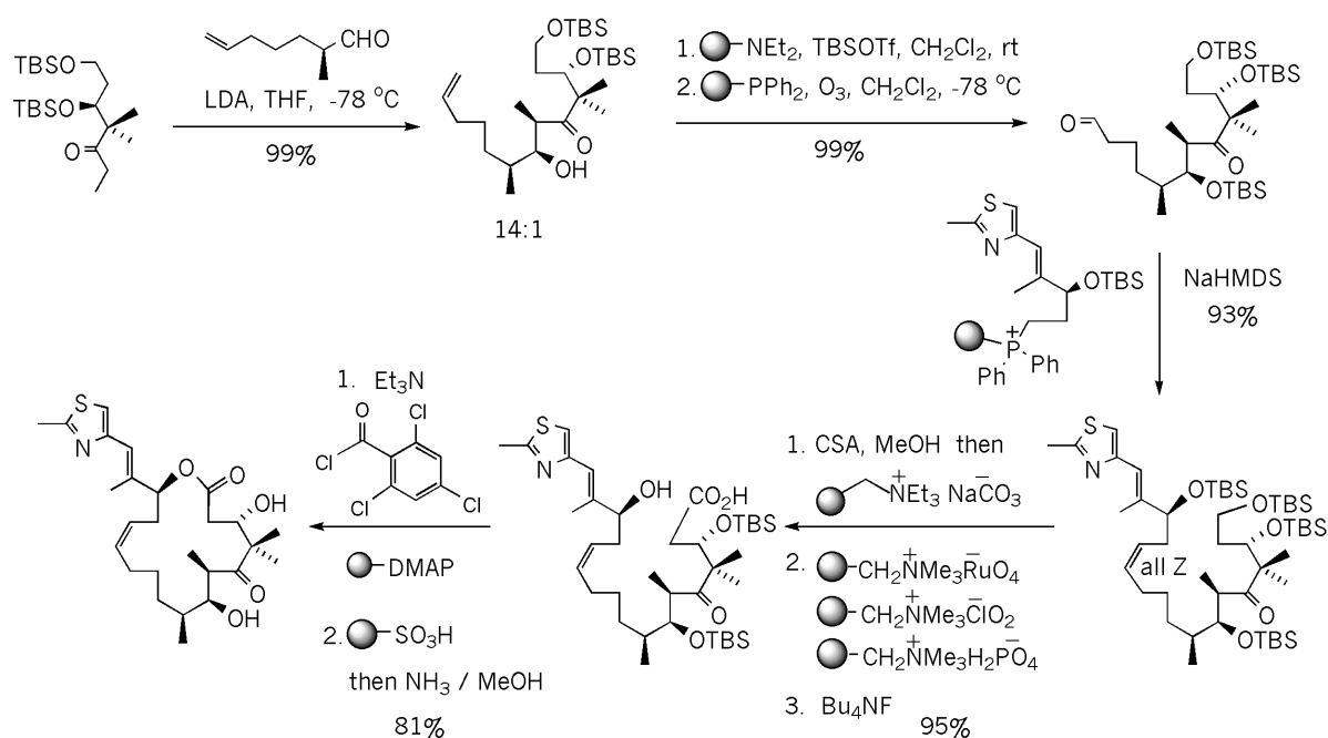
Figure 24. Final steps in the synthesis of epothilone C.
