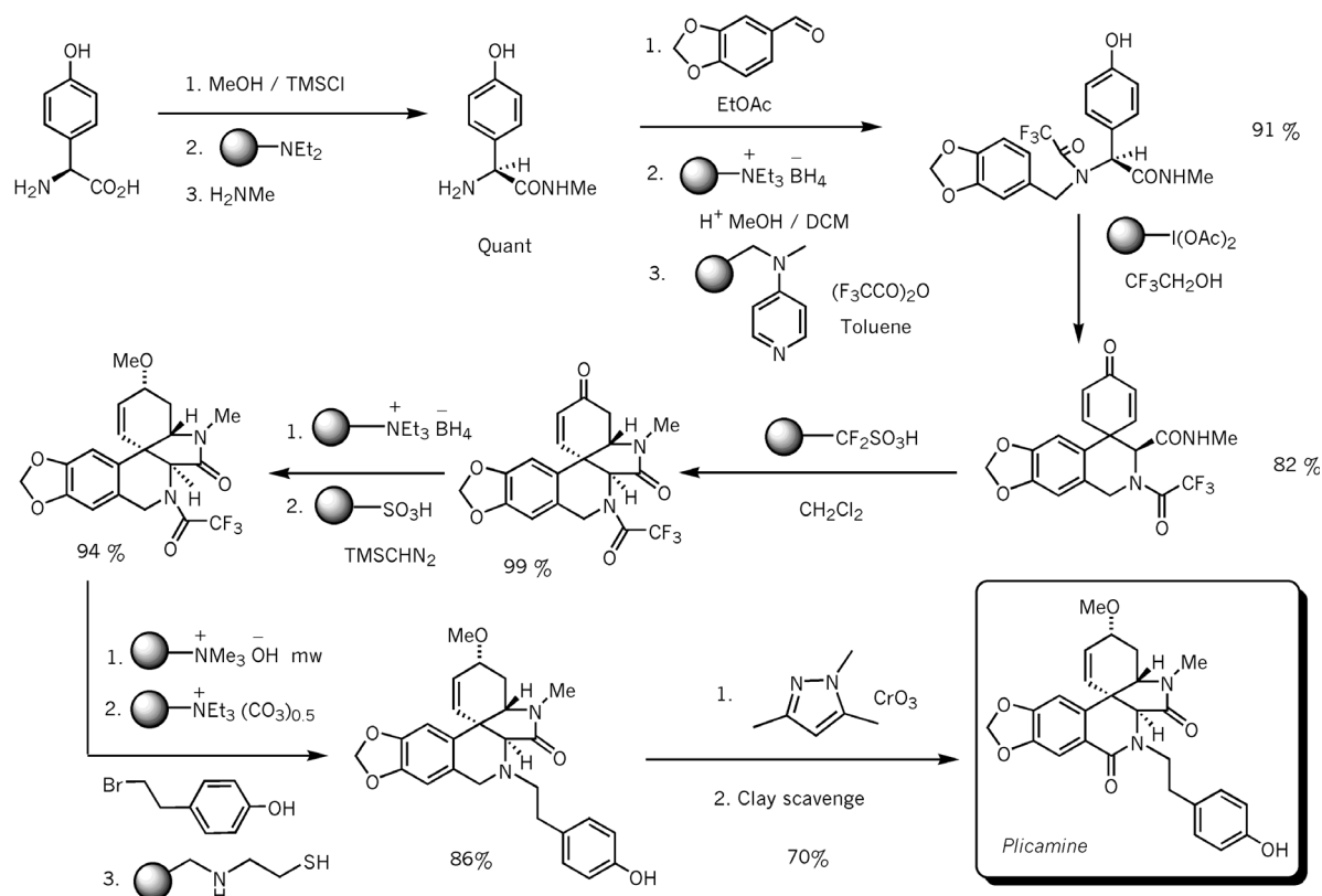
Figure 19. Synthesis of plicamine .
