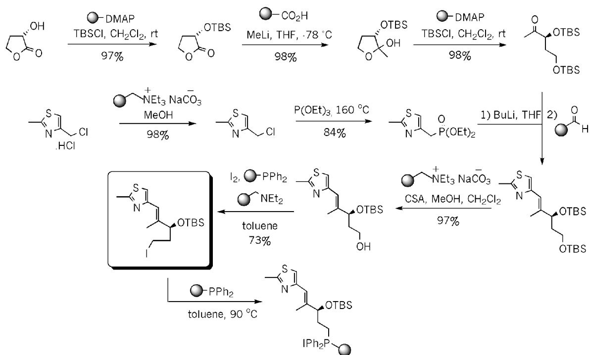
Figure 21. Synthesis of fragment A of epothilone C .
