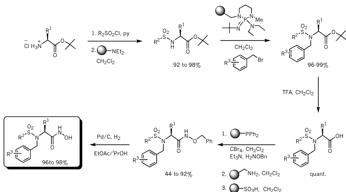
Figure 13. Synthesis of potential matrix metalloproteinase (MMP) inhibitors.
