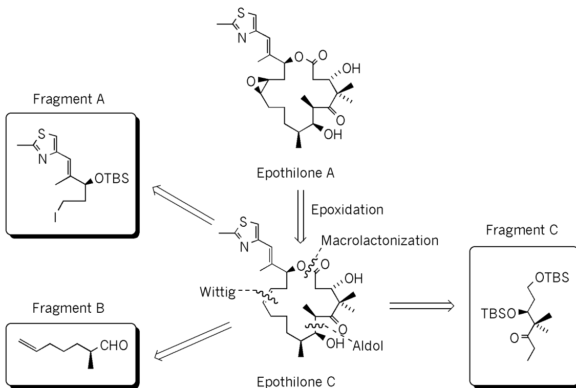
Figure 20. Synthesis of plan for epothilone C .
