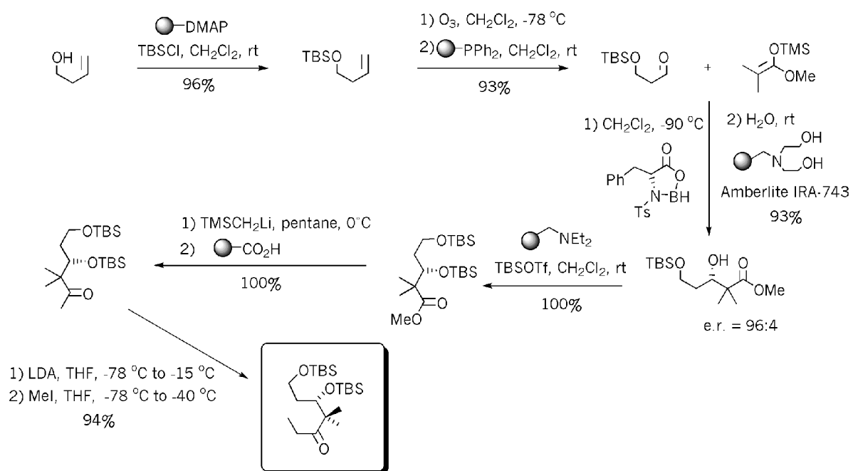
Figure 23. Synthesis of fragment C of epothilone C .
