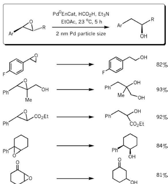
Figure 11. Pd(0) nanoparticles micro-encapsulated for the hydrogenolysis of epoxides.
