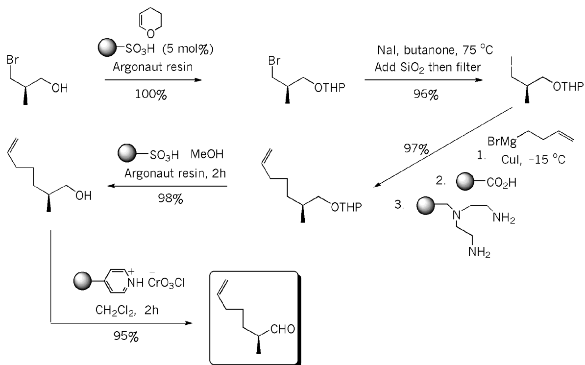
Figure 22. Synthesis of fragment B of epothilone C .
