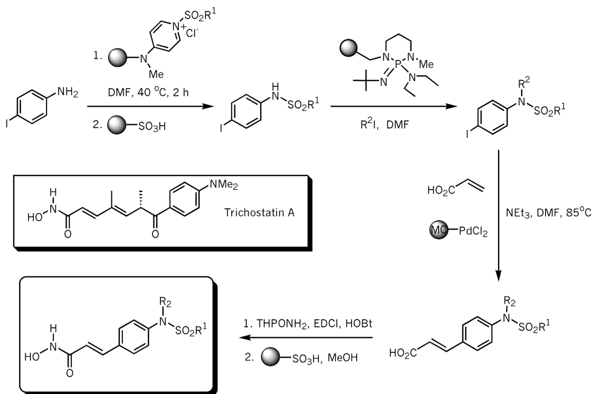
Figure 12. Synthesis of histone deacetylase inhibitors.
