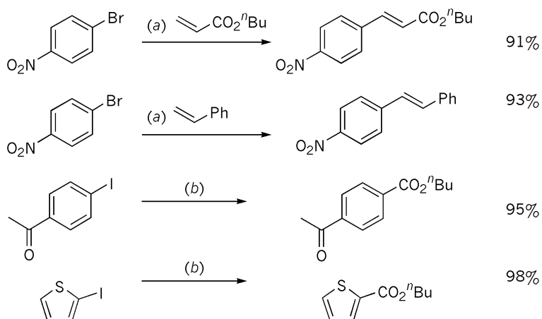
Figure 8. Conditions: (a) (Heck 2.5 mol% MC-[Pd], IPA, n\text{BuN}_4\text{OAc} , 90^\circ\text{C} plus olefin. (b) (Carbonylation) 3 mol% MC-[Pd], CO, n\text{BuOH} , \text{Et}_3\text{N} , 90^\circ\text{C} .
