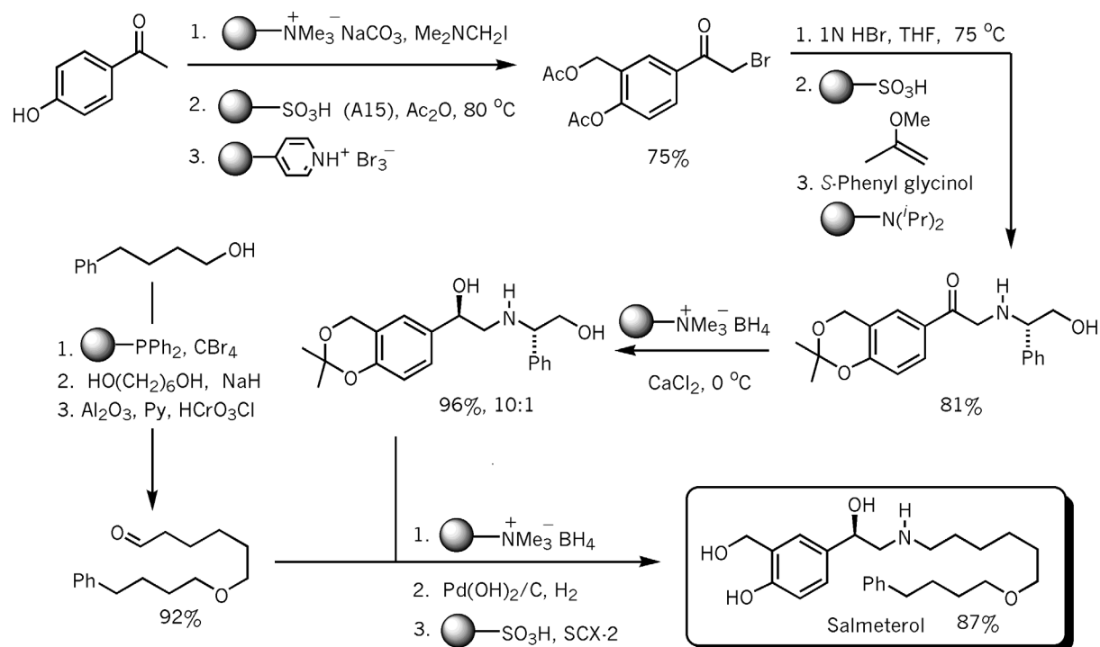
Figure 15. Synthesis of the GSK \beta_2 agonist bronchodilator salmeterol .
