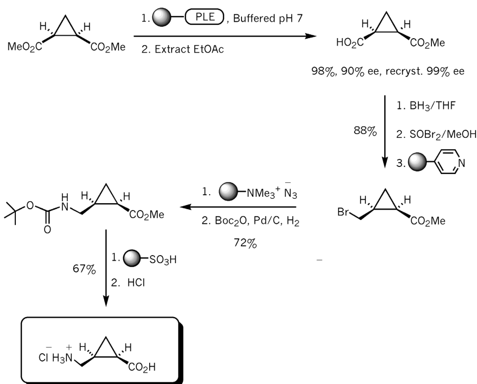
Figure 14. Using immobilised enzymes, in this case pig liver esterase (PLE), in the synthesis of GABA analogues.
