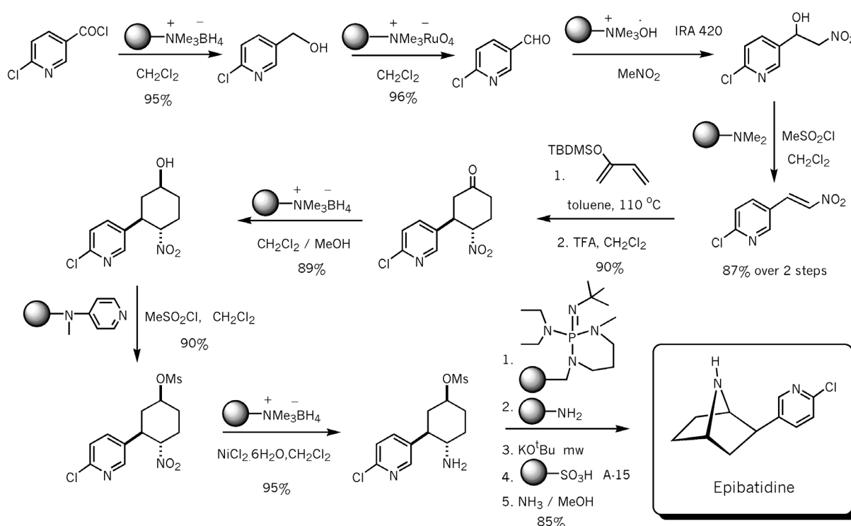
Figure 18. Synthesis of epibatidine .
