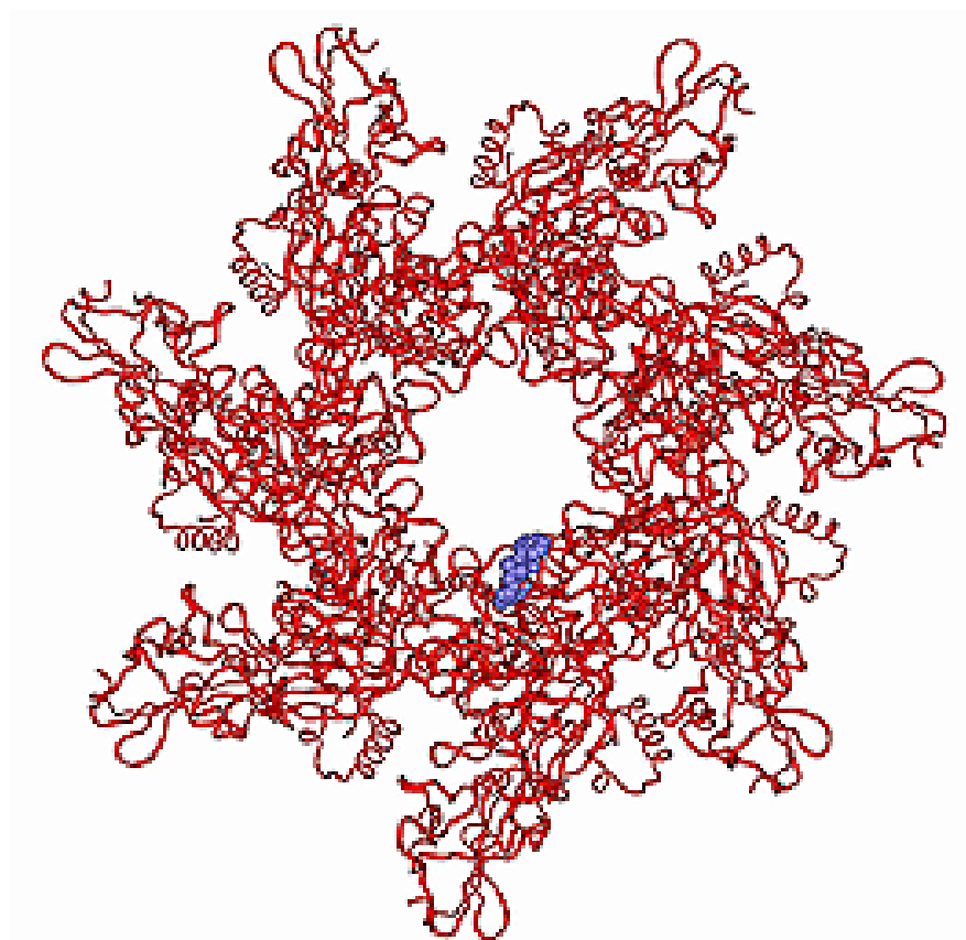
Figure 5. A detailed view of the tetrapeptide binding site of the anthrax toxin.
